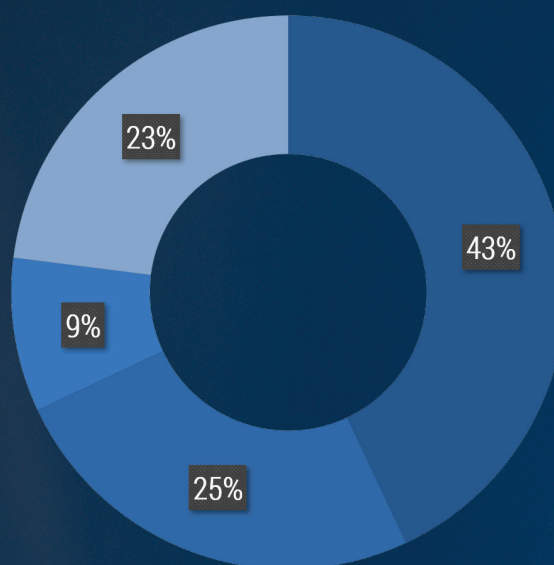
Job Title
